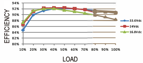
DDR-240B-48
