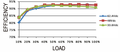
DDR-240C-48
