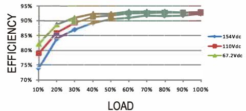
DDR-240D-48
